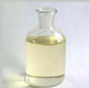
Fatty acid Methyl esters
